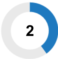
Overall Score
